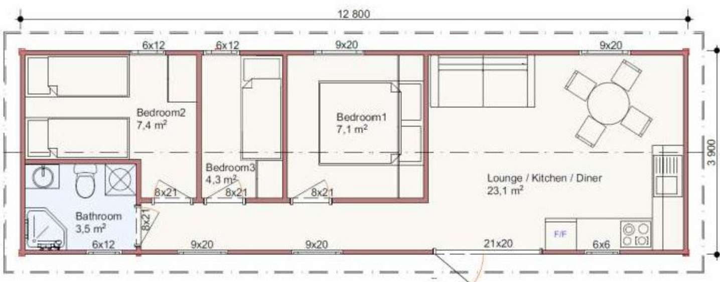
Lapwing 50 3 Bedroom - Gross Floor area-50m 2 , Living area-47m 2
