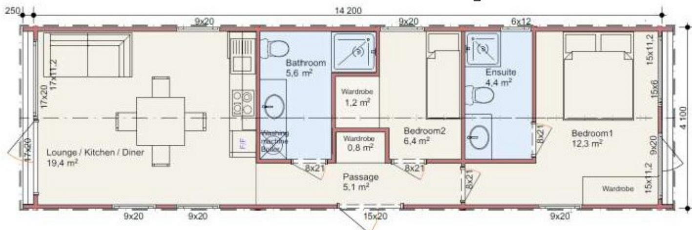
Heron 58 2 Bedroom - Gross Floor area-58m 2 , Living area-55m 2 , Deck 2m 2
